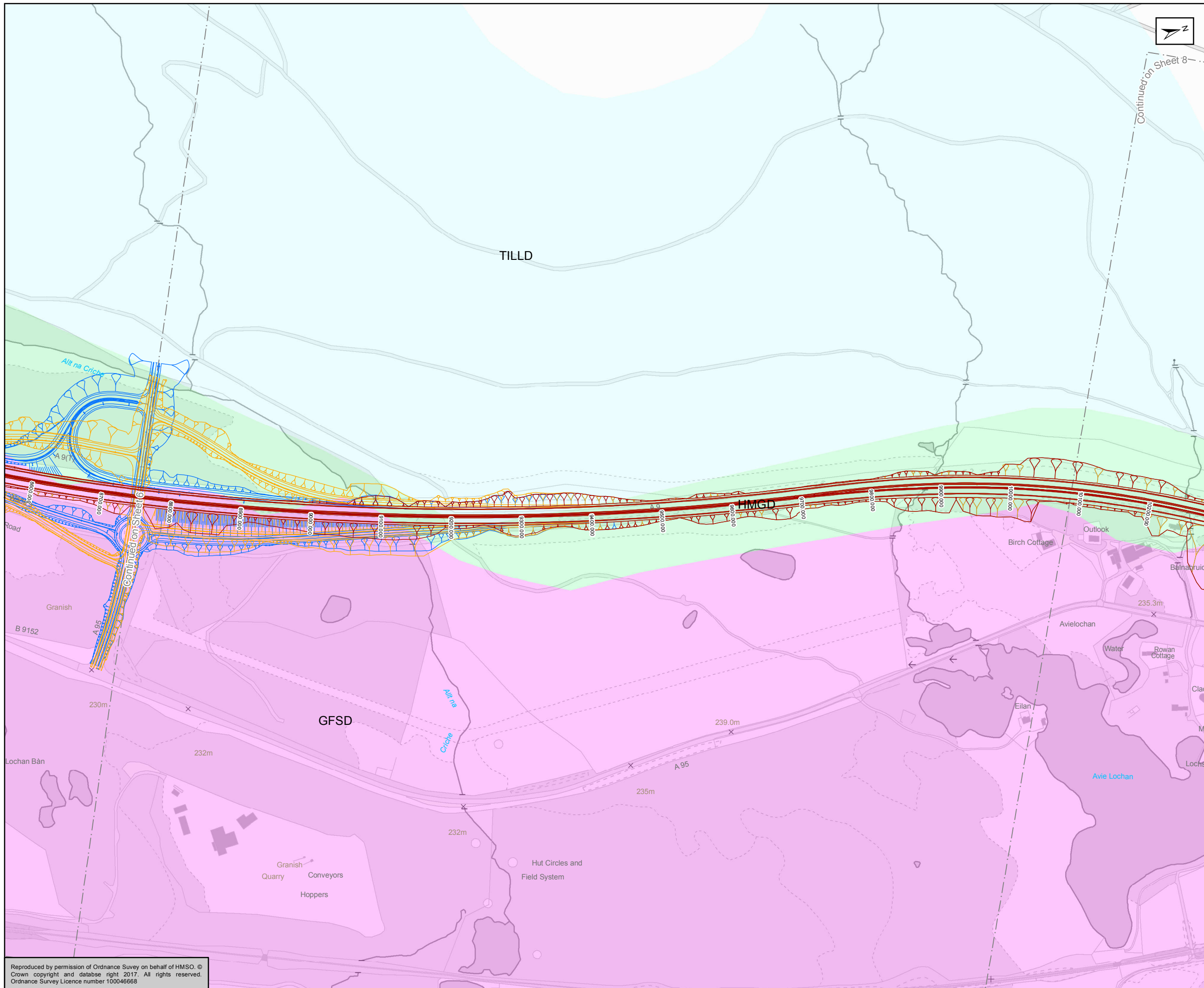
Figure 5.22g Mainline Alignment Option 1 Superficial Geology Sheet 7 of 17
