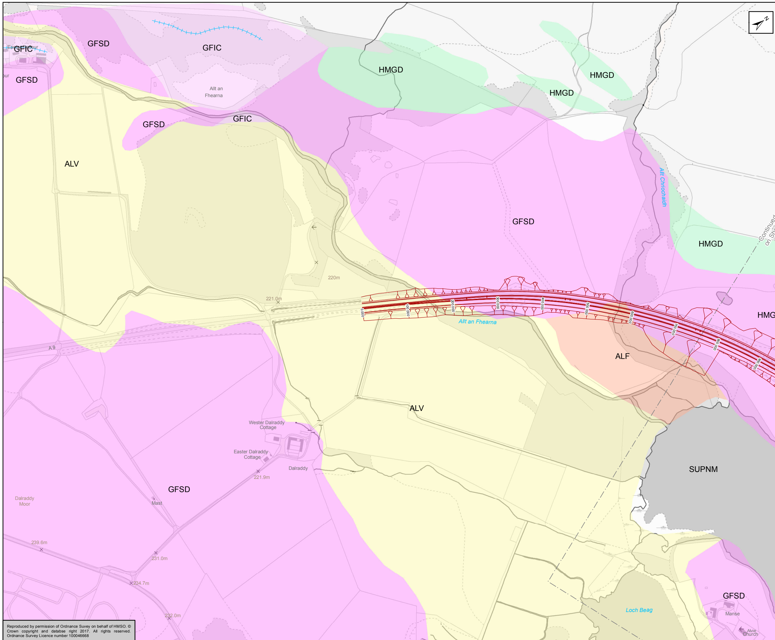
Figure 5.22a Mainline Alignment Option 1 Superficial Geology Sheet 1 of 17
