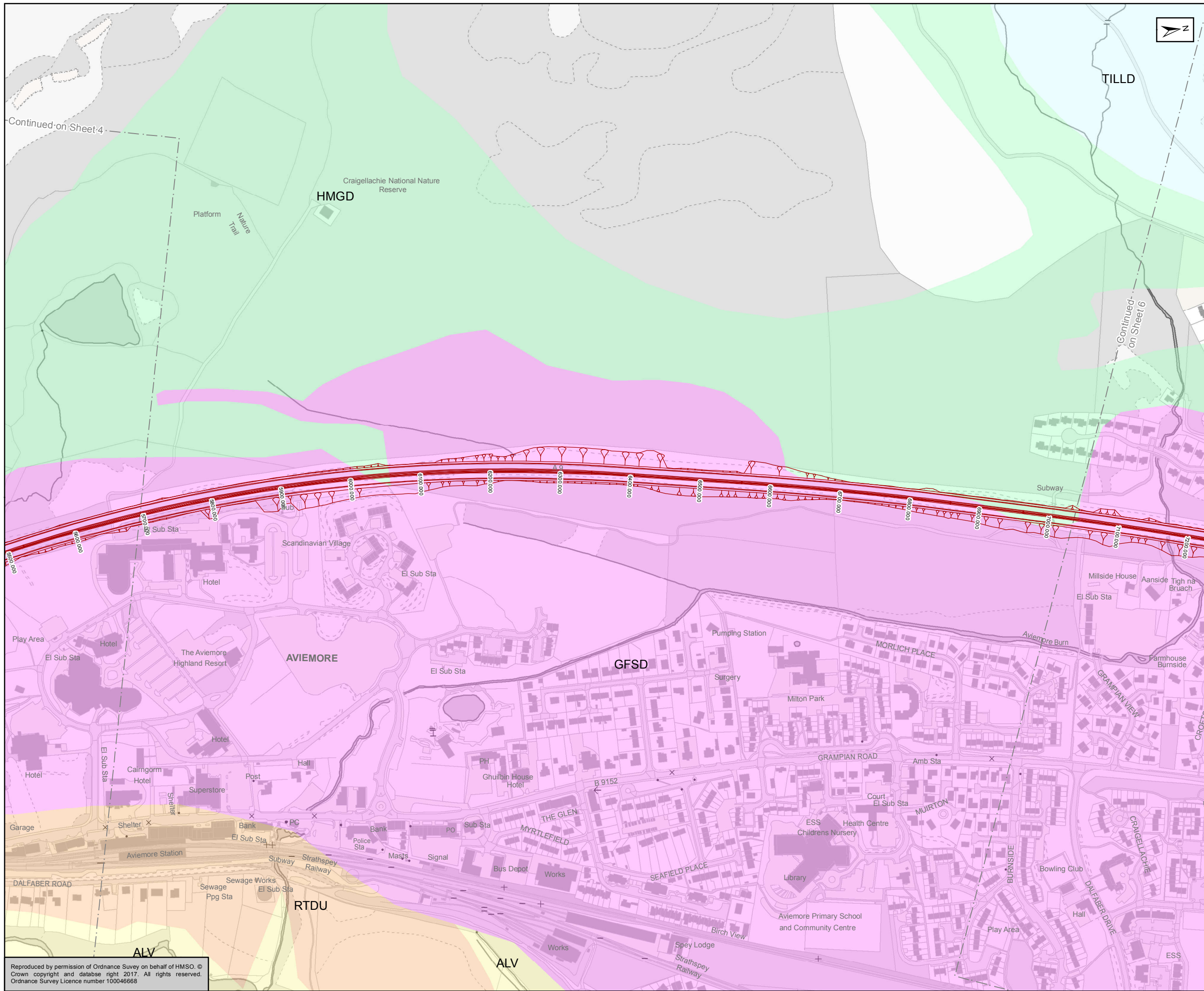
Figure 5.22e Mainline Alignment Option 1 Superficial Geology Sheet 5 of 17
