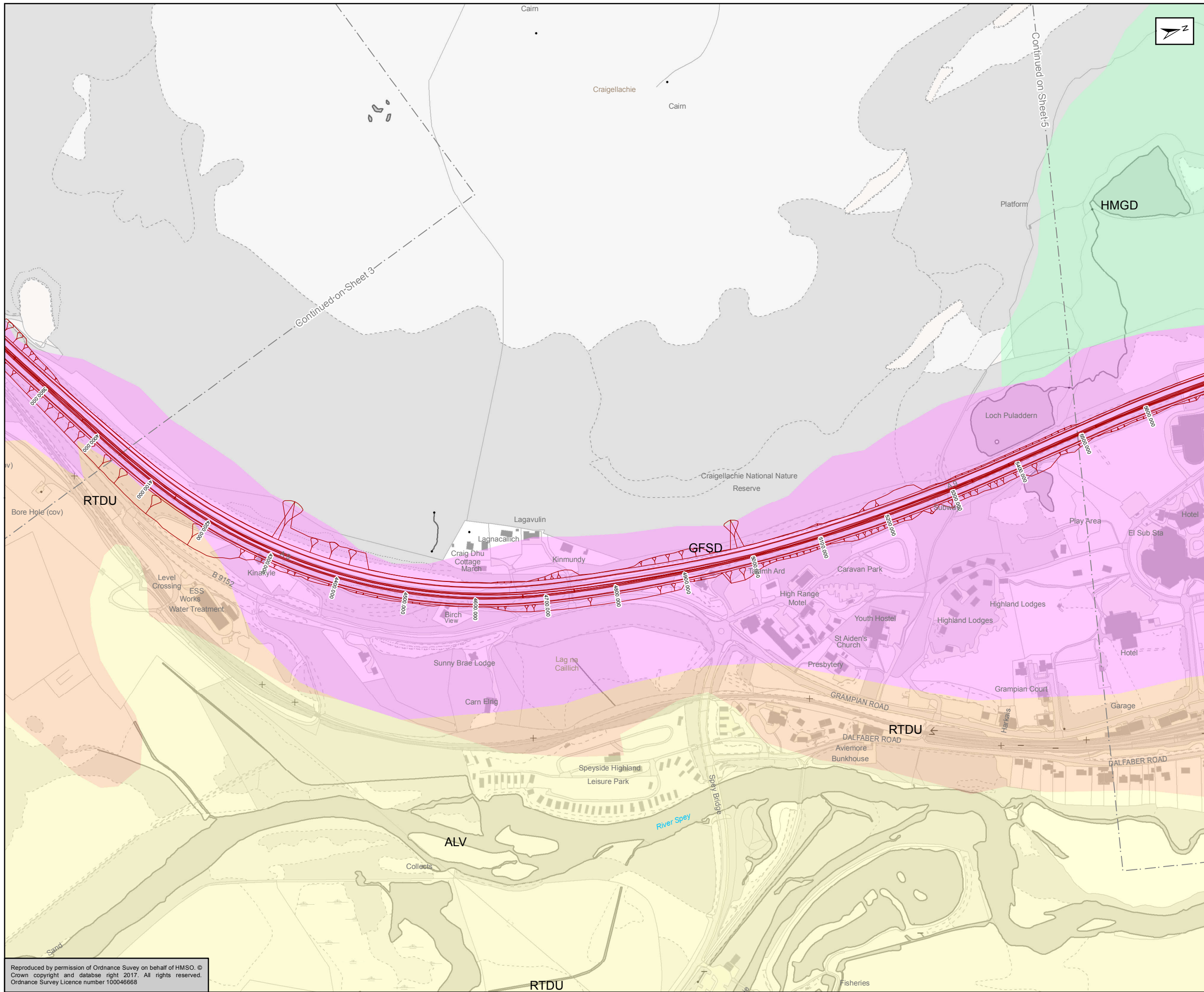
Figure 5.22d Mainline Alignment Option 1 Superficial Geology Sheet 4 of 17
