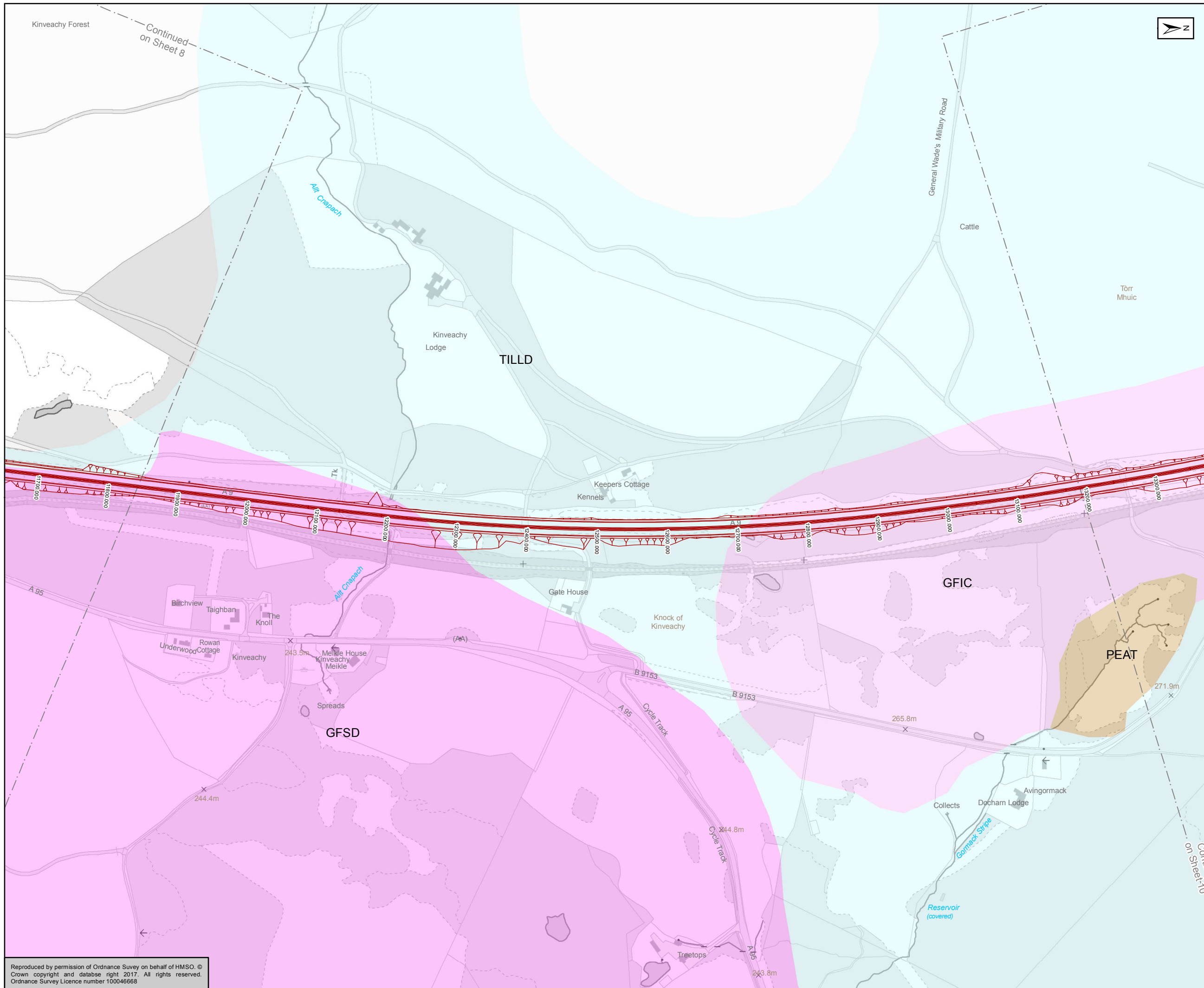
Figure 5.22i Mainline Alignment Option 1 Superficial Geology Sheet 9 of 17
