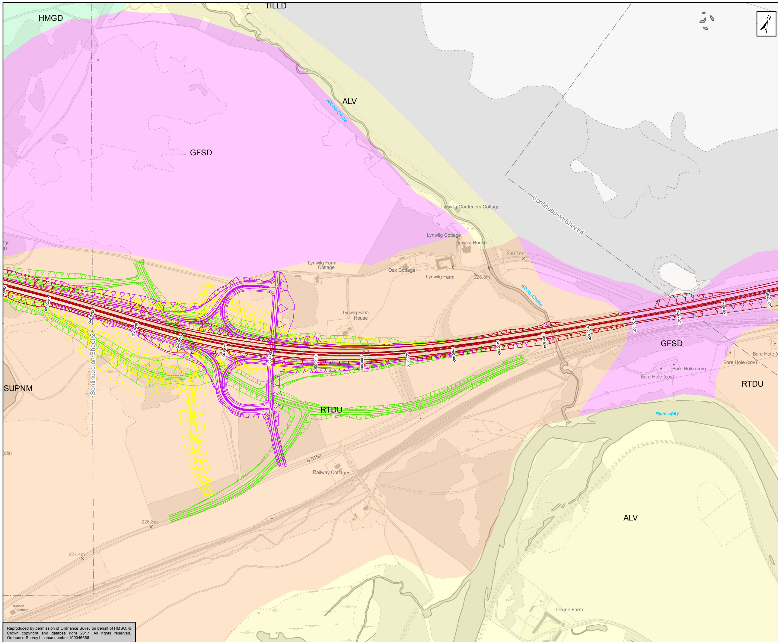
Figure 5.22c Mainline Alignment Option 1 Superficial Geology Sheet 3 of 17
