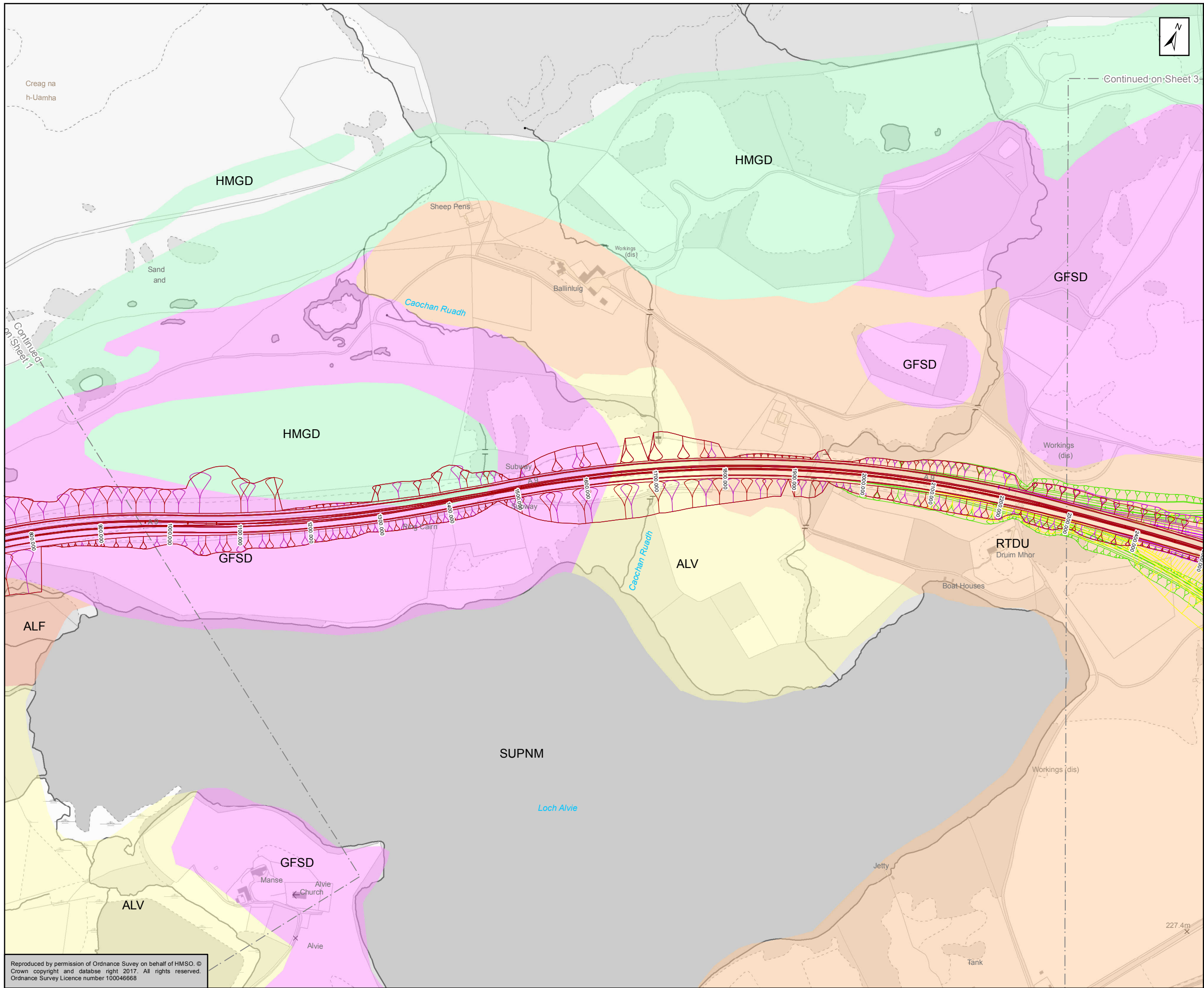
Figure 5.22b Mainline Alignment Option 1 Superficial Geology Sheet 2 of 17
