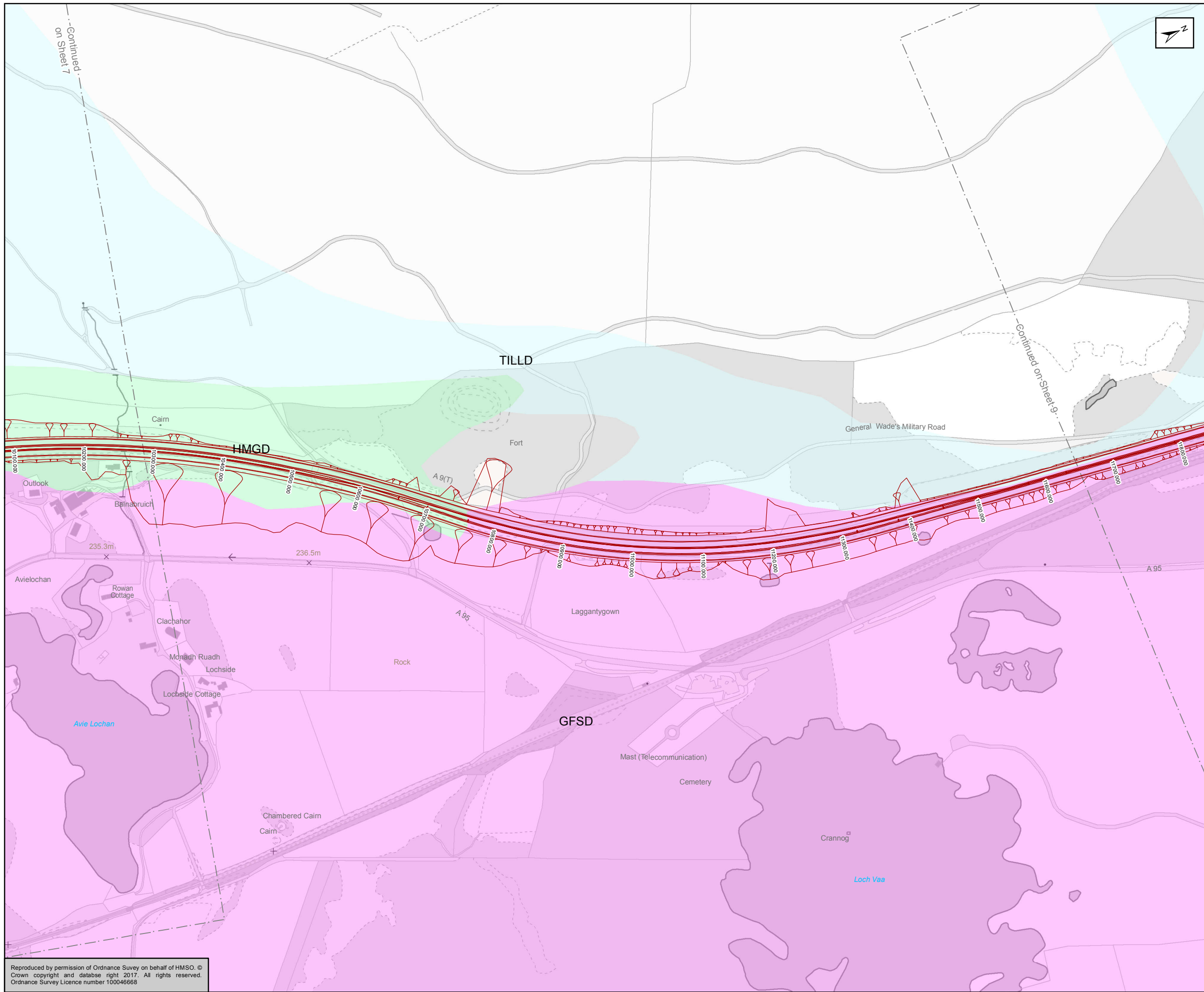
Figure 5.22h Mainline Alignment Option 1 Superficial Geology Sheet 8 of 17
