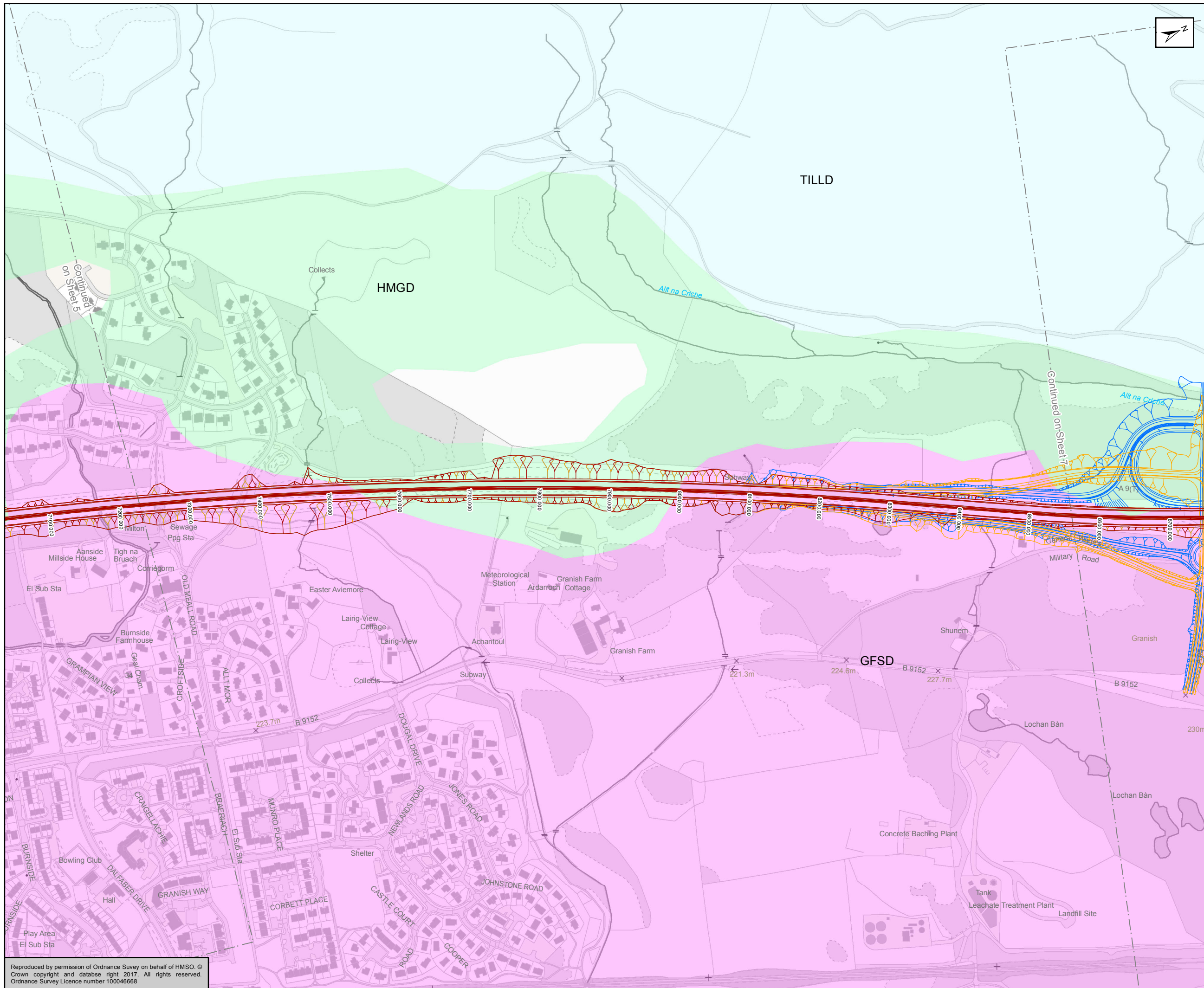
Figure 5.22f Mainline Alignment Option 1 Superficial Geology Sheet 6 of 17
