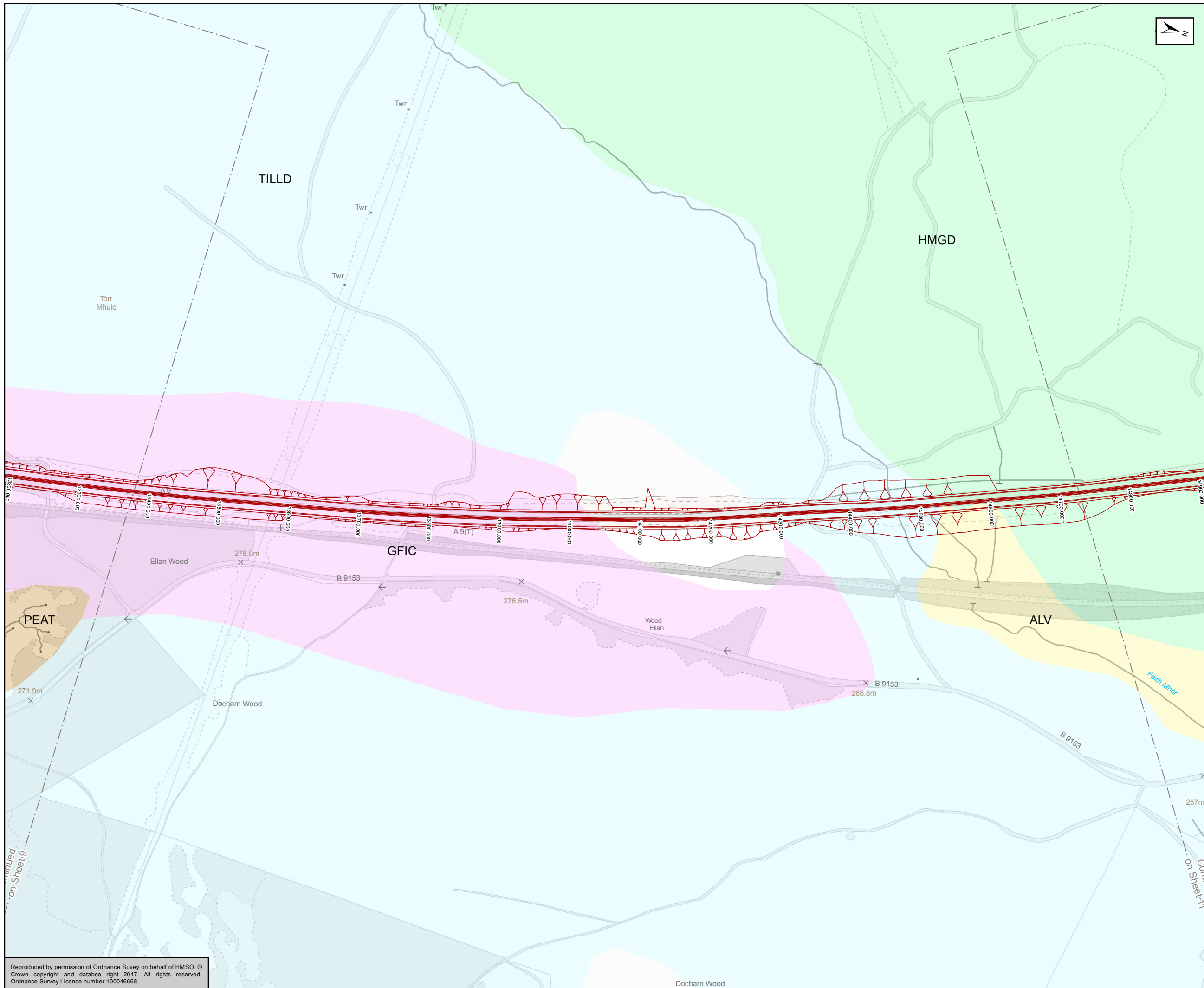
Figure 5.22j Mainline Alignment Option 1 Superficial Geology Sheet 10 of 17
