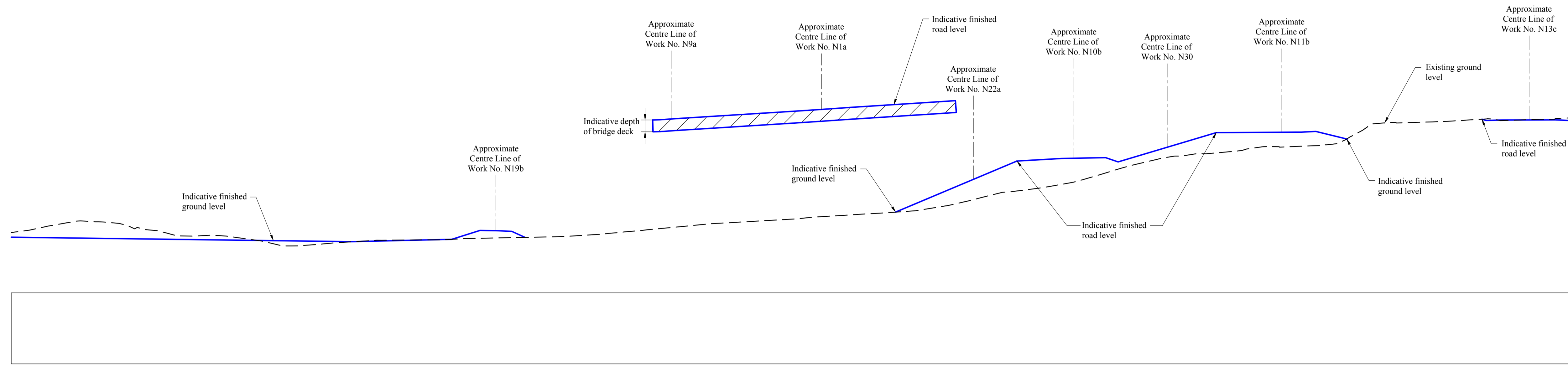
Indicative Cross-section X14A - X14A Scale 1/500
