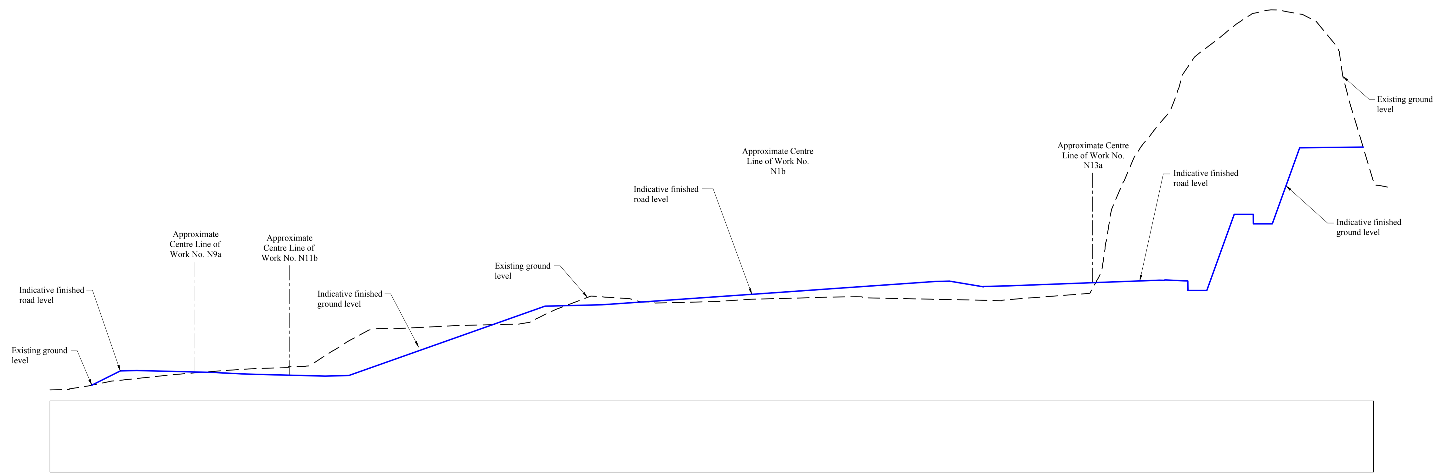
Indicative Cross-section X14B - X14B Scale 1/250
