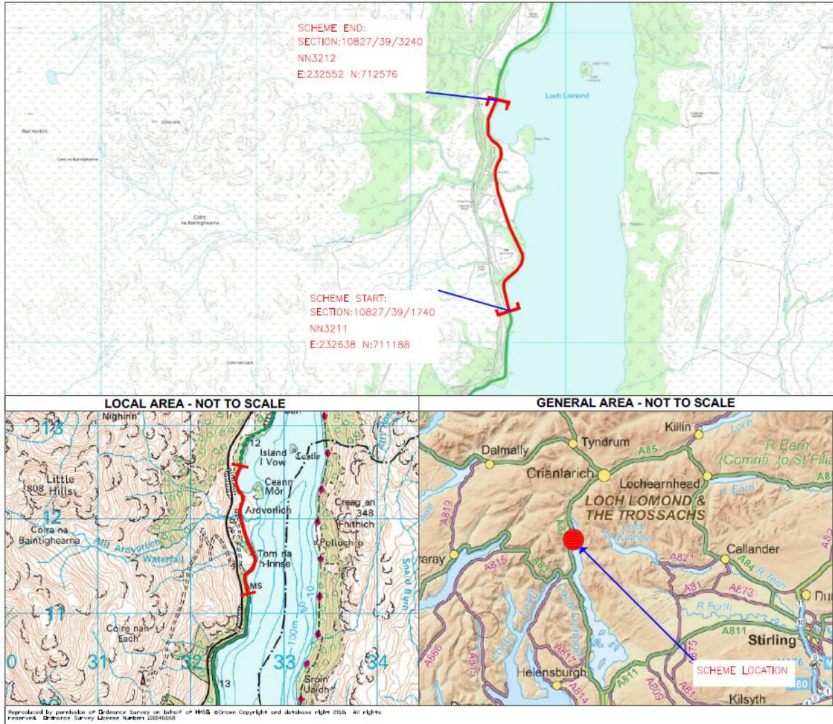
Figure 1. Location and scheme extent of the proposed resurfacing works at A82 Ardvorlich to Pulpit Rock. Source: BEAR Scotland.
