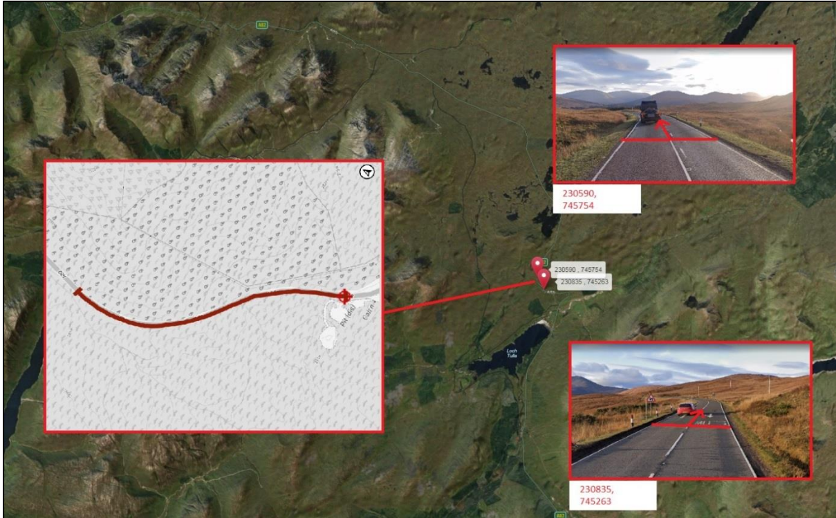
Figure 1. Location and scheme extent of the proposed resurfacing works at A82 North of Loch Tulla Viewpoint. Source: BEAR Scotland.
